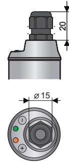
Variant "D" with dustproof cable outlet
