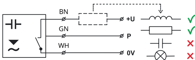
connecting the sensor with programming wire (version W)
