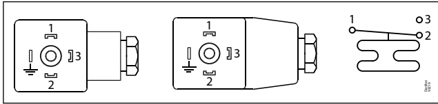
Figure 1: Electrical connection
